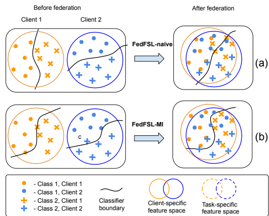
Fig. 4: Illustration of decision boundaries learned by (a) FedFSL-naive and (b) FedFSL-MI in two-client case.
