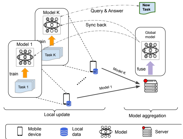
Fig. 1: Overview of a FedFSL system. Distributed client devices train models with sampled FSL tasks, send the models to the central server to aggregate for a central model, and synchronize back for the next round of local updates.
